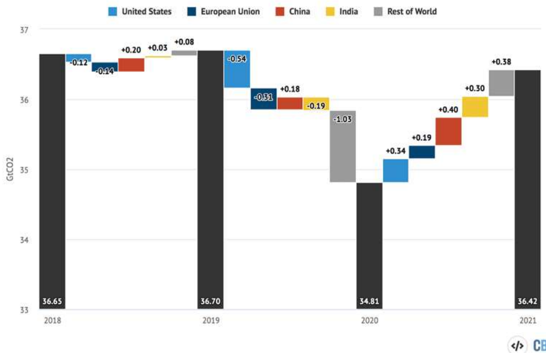
Change in global emissions from fossil fuels by country, 2018-2021
