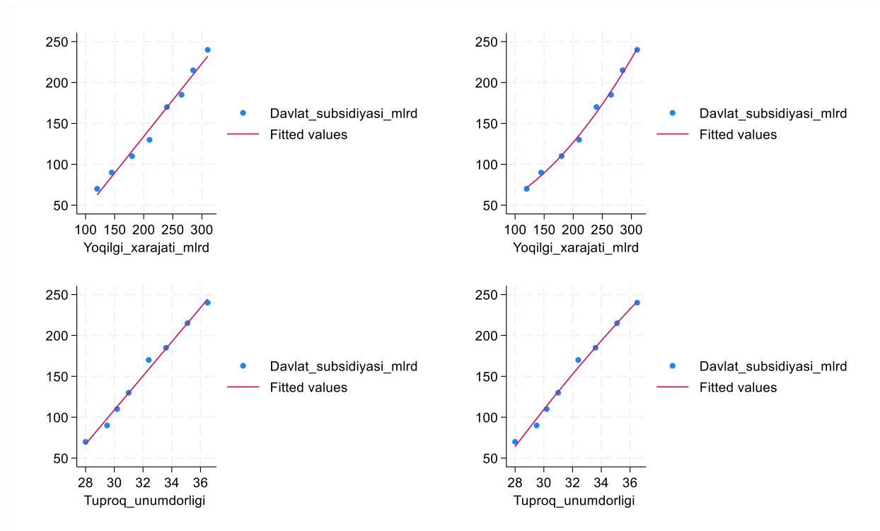
2-rasm. O'zgaruvchilar chiziqli munosabatining scatterplot chizmasi
