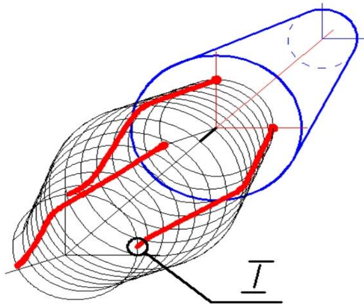
1-rasm. Yumshatkich ishchi organining murakkab geometrik sirtini qurish.
