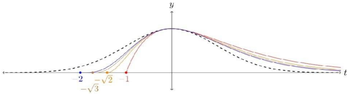
FIGURE 2. Plot of |f_n| = f_n for 1 \leq n \leq 4 and y = e^{-t^2/2} .
